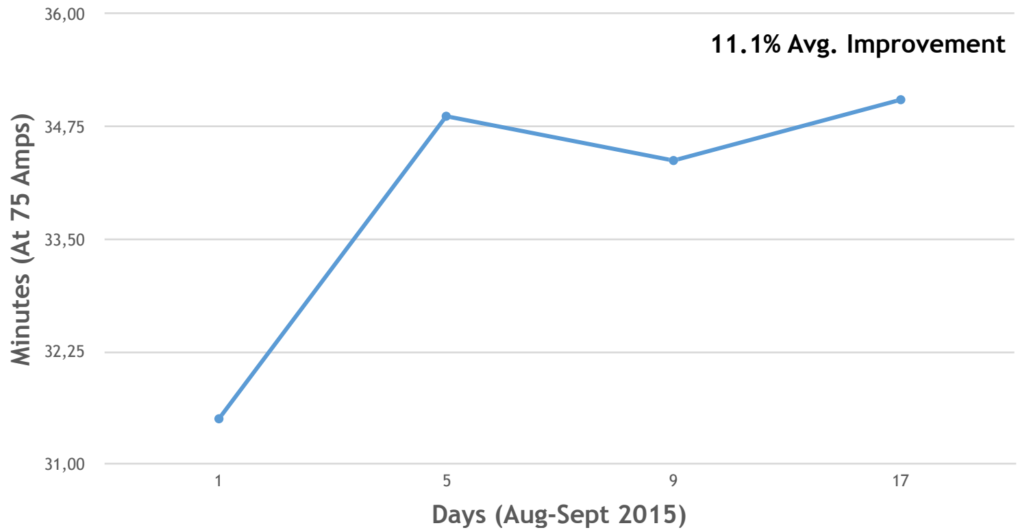
Load Test Results (Avg. Batteries 1-6)
